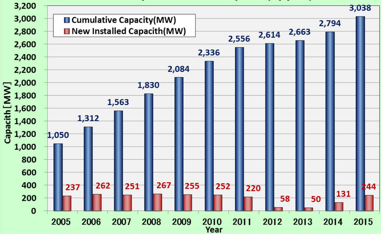
Wind power installed capacith(By year)
